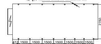
Base vibration absorption installation diagram 16-φ14 vibration absorption installation hole
